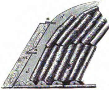
Fig. 315.—Plank-supports of Alpine kiln.
